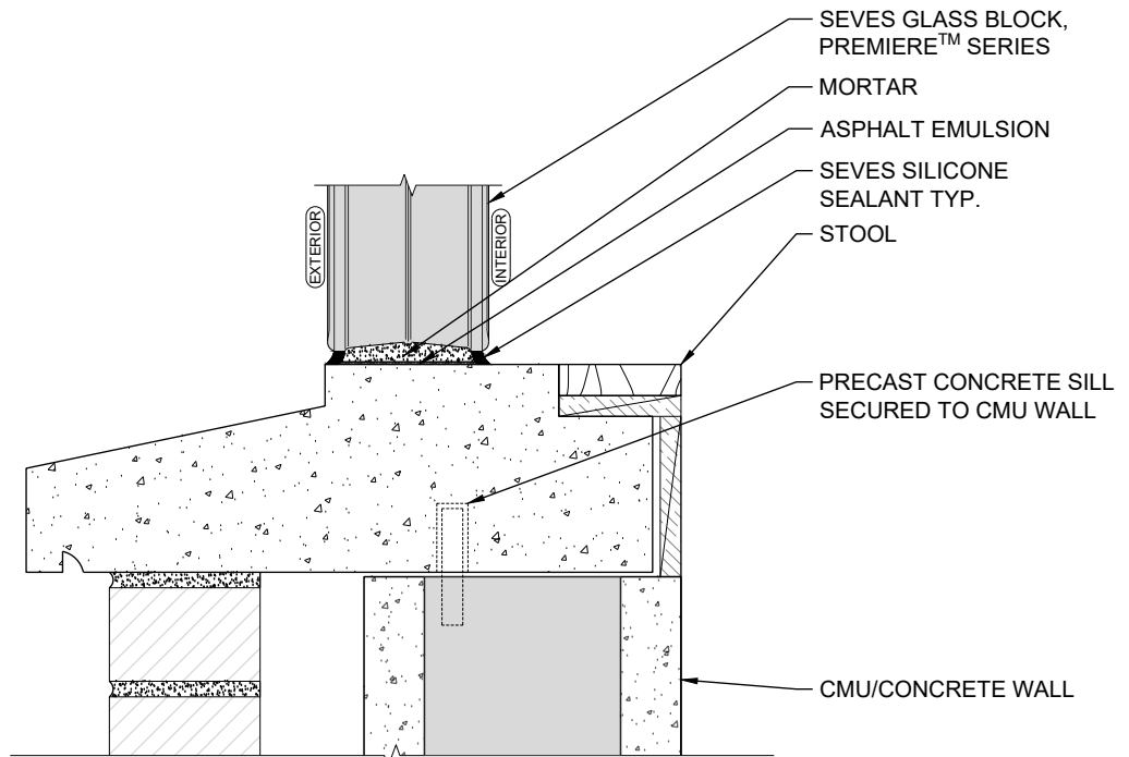
SILL - 45 MIN FIRE RATED GLASS BLOCK IN CMU/CONCRETE WALL SCALE: N.T.S.
