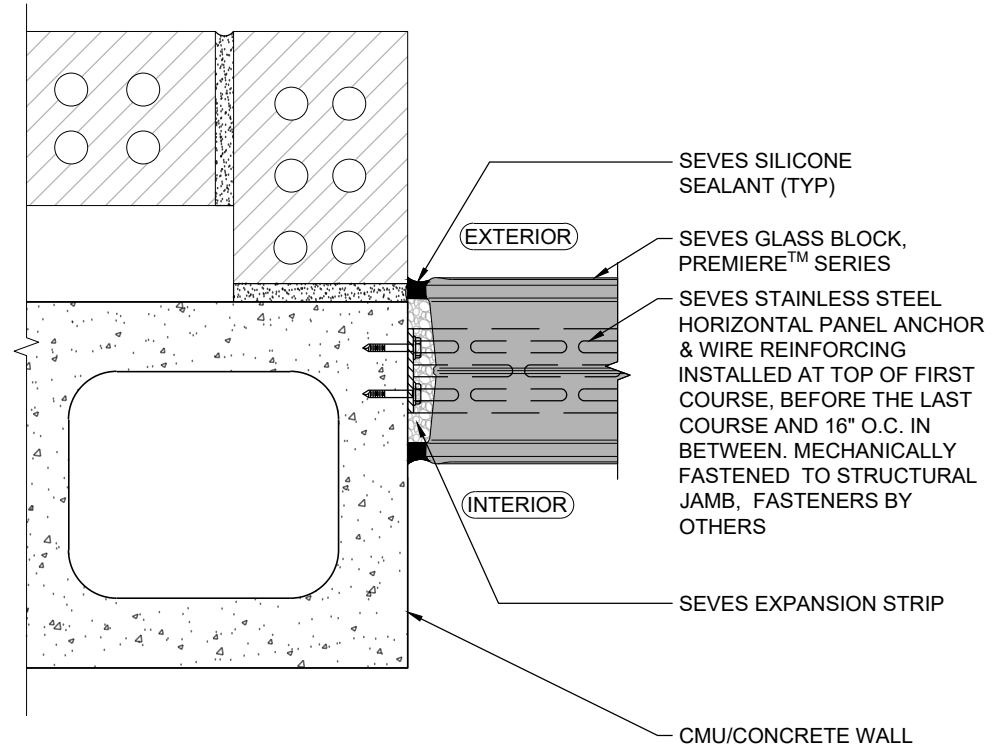
JAMB - 45 MIN FIRE RATED GLASS BLOCK IN CMU/CONCRETE WALL
