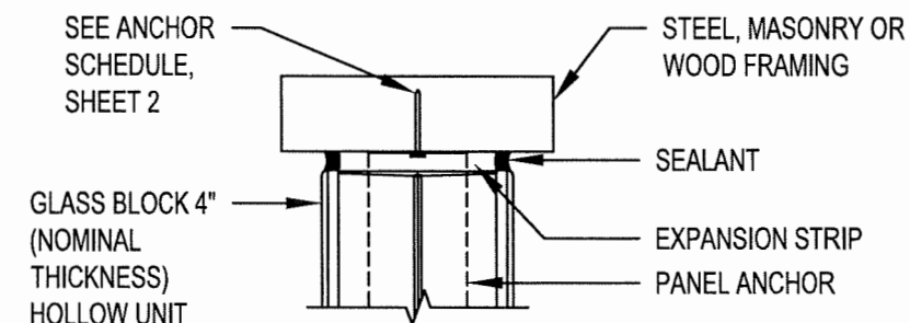
PANEL ANCHOR RESTRAINT DETAIL SCALE: 3" = 1'-0"
