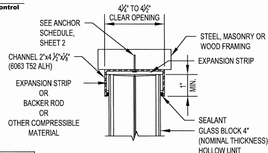
CHANNEL RESTRAINT DETAIL SCALE: 3" = 1'-0"
