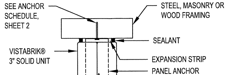
PANEL ANCHOR RESTRAINT DETAIL SCALE: 3" = 1'-0"
