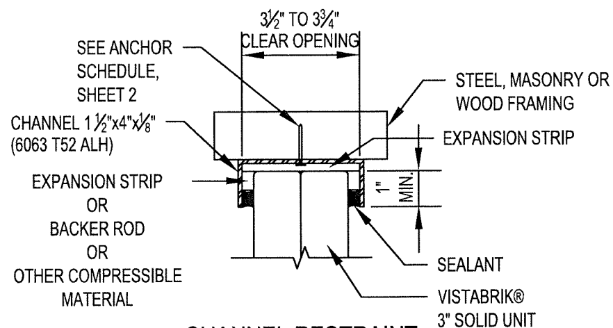
CHANNEL RESTRAINT DETAIL SCALE: 3" = 1'-0"
