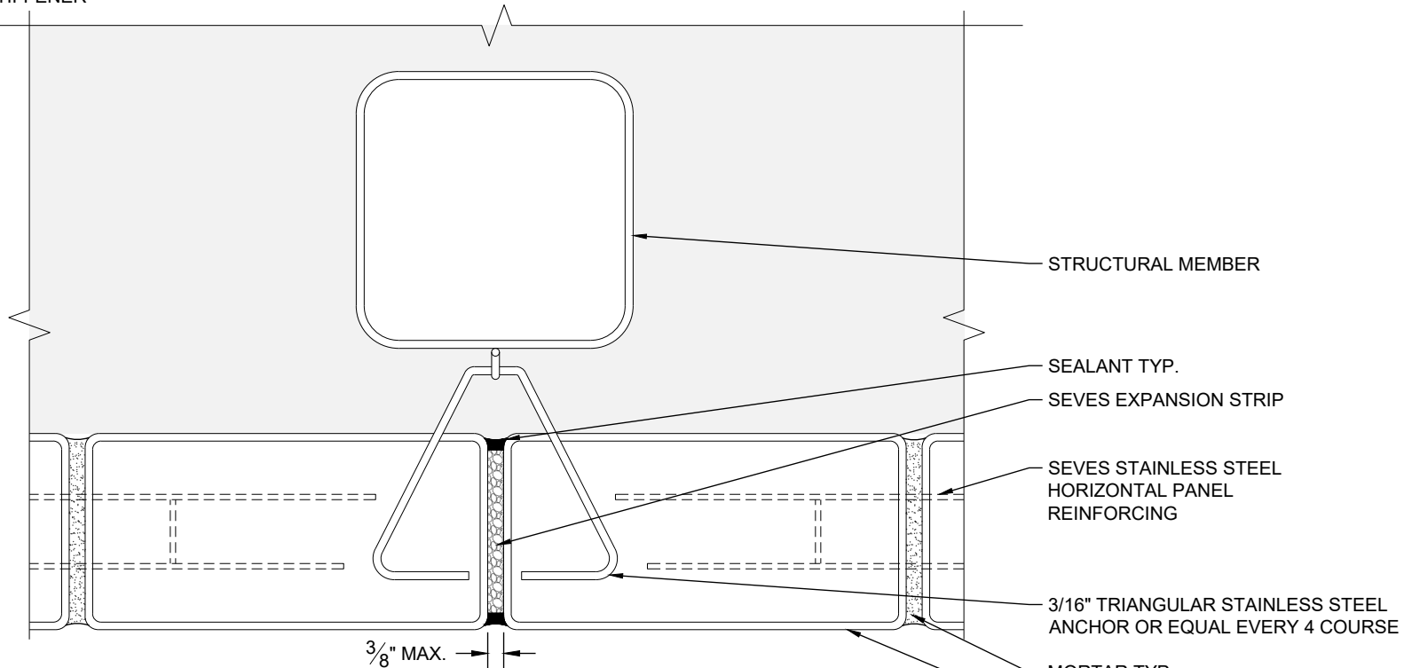
VERTICAL STIFFENER
