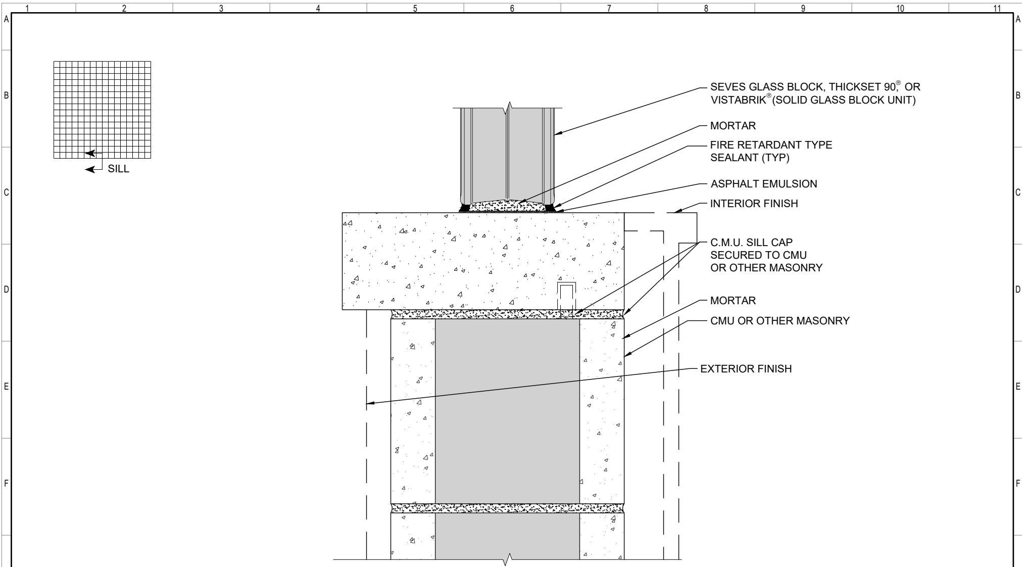
SILL - 90 MIN FIRE RATED GLASS BLOCK AT CMU WALL
