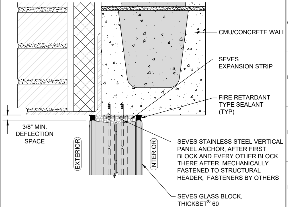
HEAD - 60 MIN FIRE RATED GLASS BLOCK IN CMU/CONCRETE WALL
